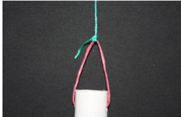
EXAMPLE OF A CENTRALLY HUNG POLE WITH A DRILLED HOLE. THE PULLER LINE IS TIED TO A SEPARATE LOOP WHICH PASSES THROUGH THE DRILLED HOLE. (LOOP KNOT HAS BEEN PULLED INSIDE THE HOLE).
